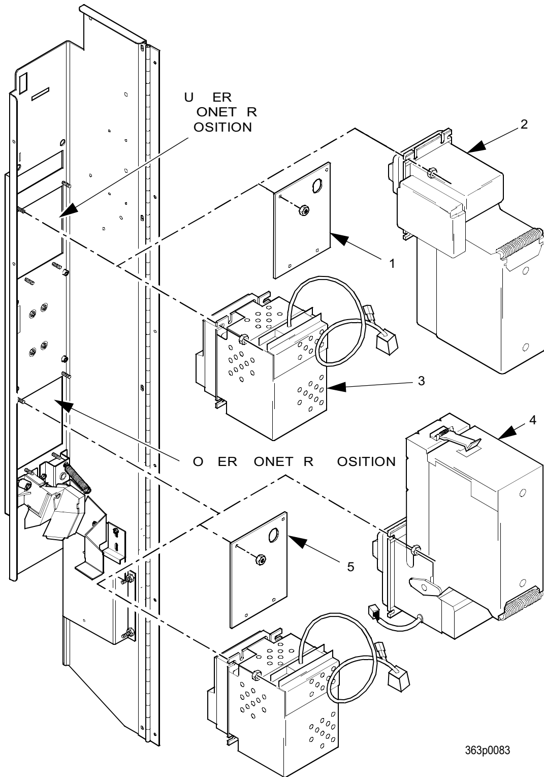
Figure 45. Card Reader and Bill Validator Combinations
