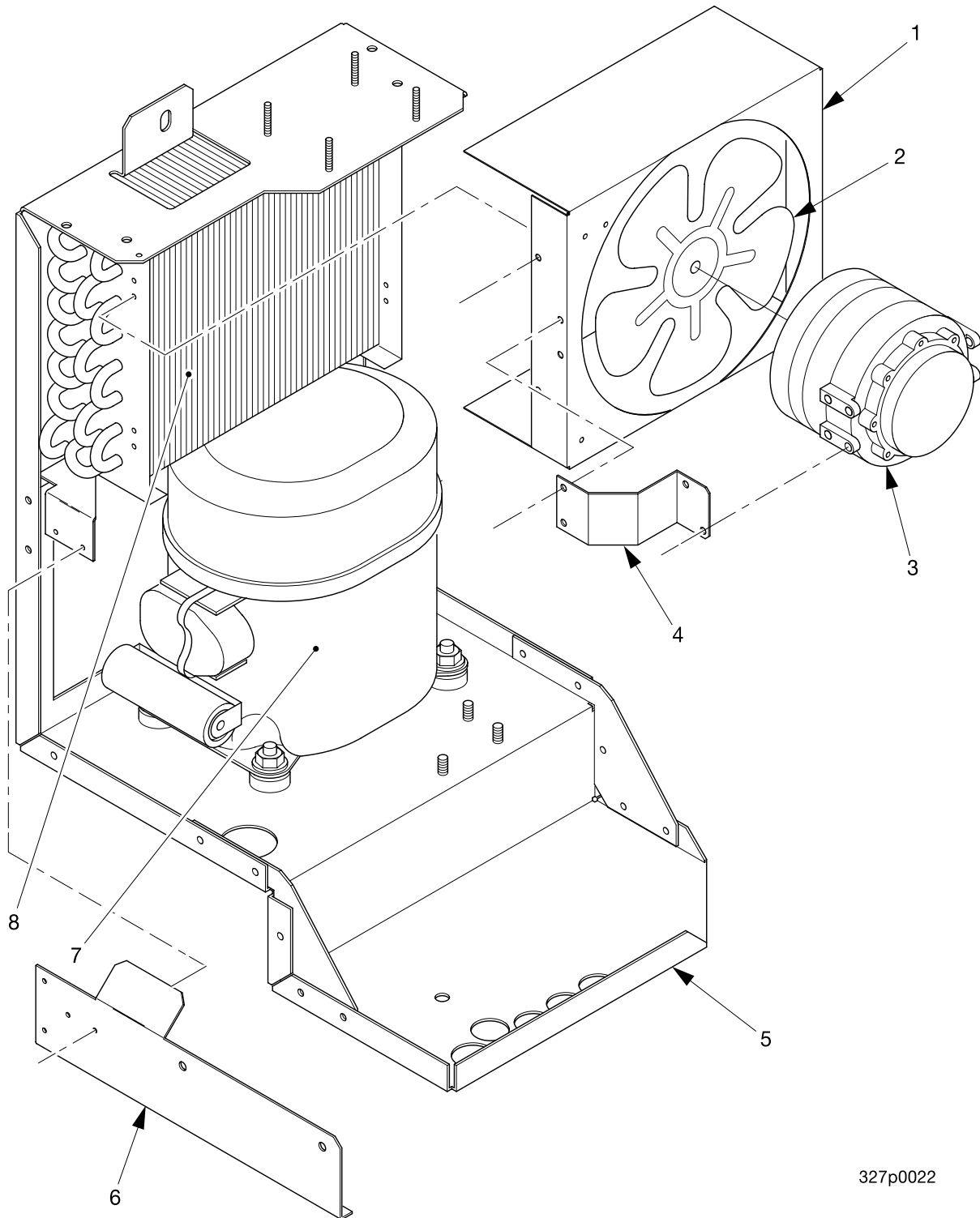
Figure 61. Icemaker Assembly - Part 8
