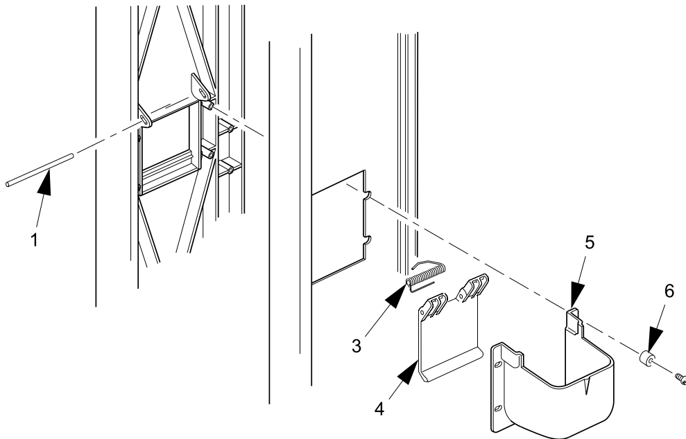
COIN RECEPTACLE ASSEMBLY - MILLINIUM
